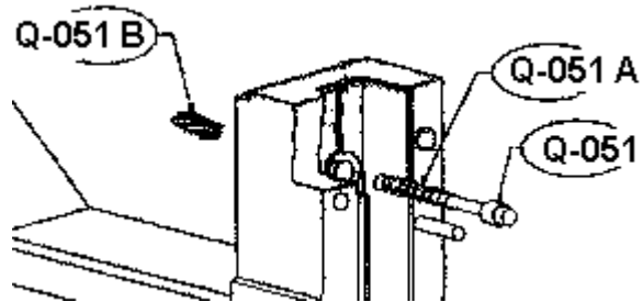
Spring-Pin system
